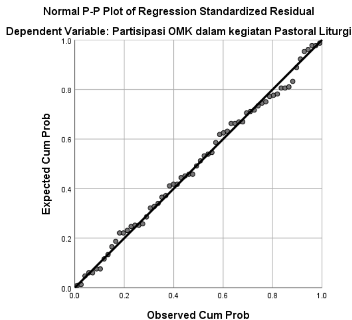
Gambar 8. Normal Probability Plot
